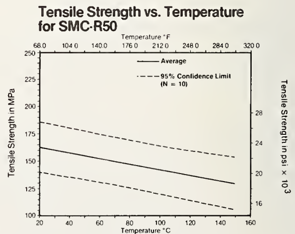
Fig. 8 - Tensile strength versus temperature for SMC-R50
